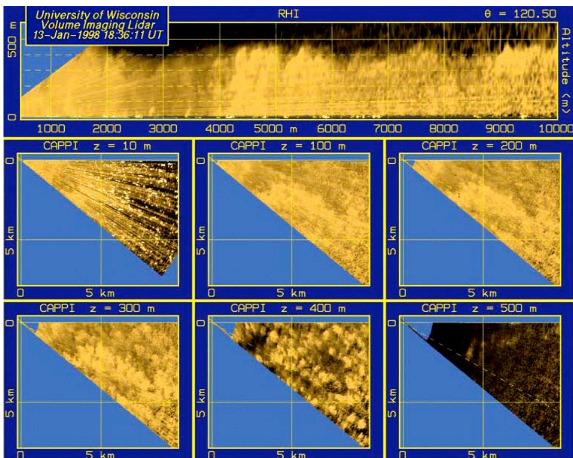
Figure 2.6: An example of Range-Height Indicator (RHI) volume scan imagery. Note that in the top image, the vertical axis is elevation from ground level and the horizontal axis represents horizontal range, similar to an RHI. The bottom images show constant altitude plane-parallel indicator (CAPPI) scans at six elevations. This particular image is from 13 January 1998.
